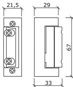
NC electric strike (normally closed) 12V DC 0.4A
